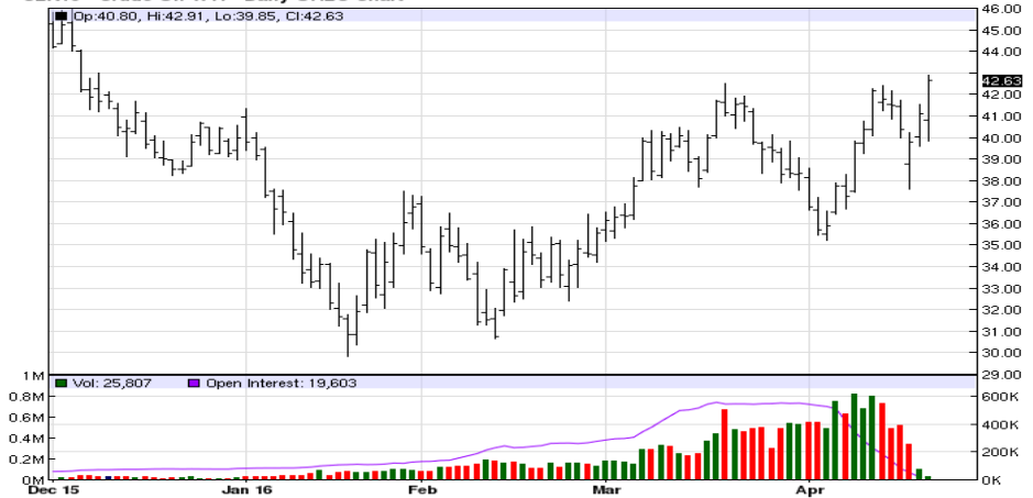
CLK16 - Crude Oil WTI - Daily OHLC Chart
